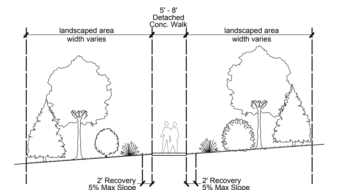
Typical Sweetgrass Low Impact Trail scale: NTS
