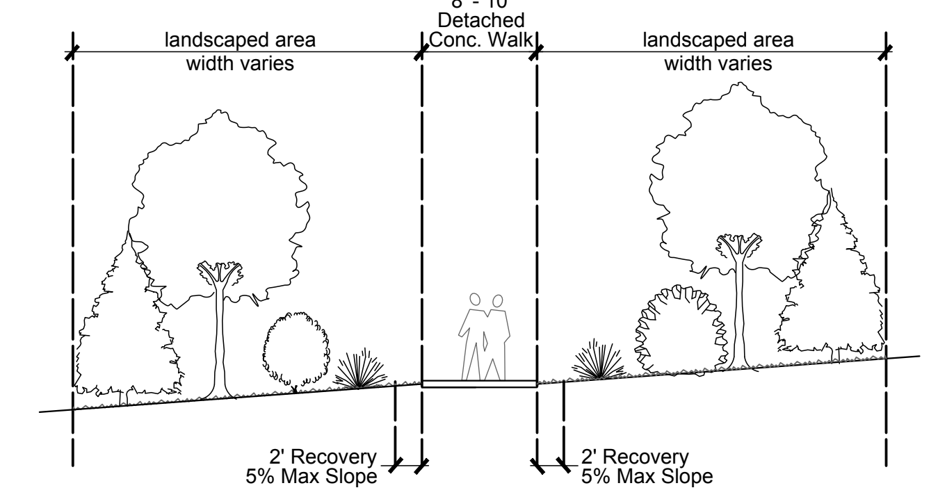
Typical Sweetgrass Regional Trail scale: NTS
