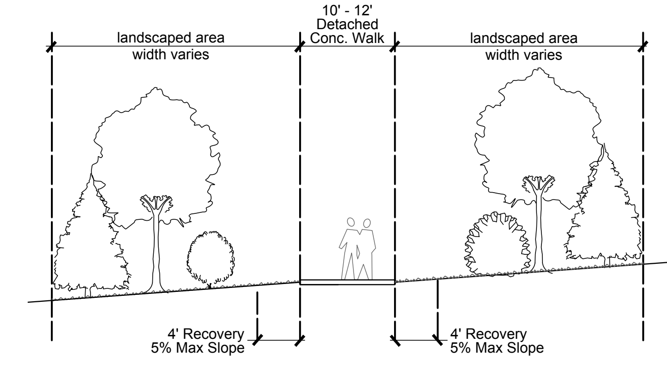
Typical Cheyenne Greenway Trail scale: NTS
